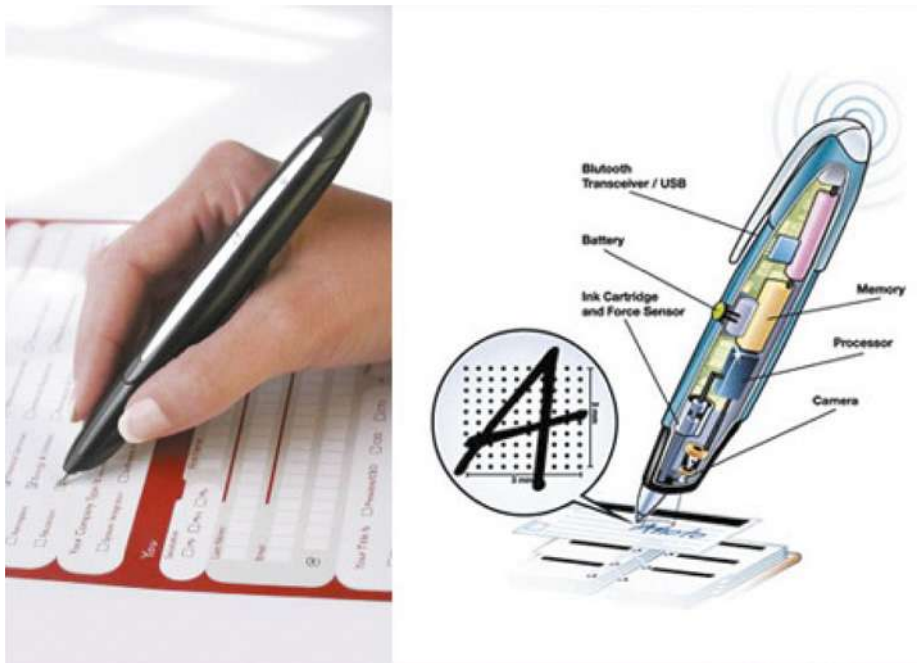
Figure 7.18 The Anoto pen being used to fill in a paper form and a schematic showing its internal components
